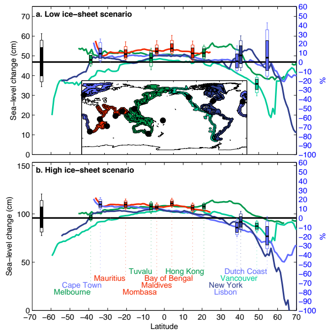
Figure 32: Sea-level rise in a 4°C warmer world by 2100 along the world’s coastlines, from South to North. Each color line indicates an average over a particular coast as shown in the inlet map in the upper panel. The scale on the right-hand side represents the ratio of regional sea-level compared to global-mean sea level (units of percent), and the vertical bars represent uncertainty thereof, showing 50 percent, 68 percent, and 80 percent ranges.
