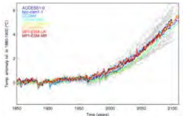
Figure A2.1: Simulated historic and 21st century global mean temperature anomalies, relative to the pre-industrial period (1880–1900), for 24 CMIP5 models based on the RCP8.5 scenario. The colored (and labeled) curves show those simulations reaching a global mean warming of 4°C–5°C warmer than pre-industrial for 2080–2100, which are used for further analysis.
